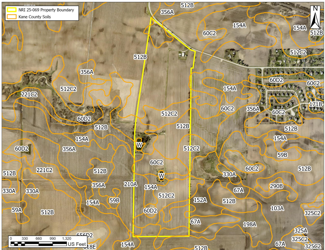
Figure 11: Soil Survey
